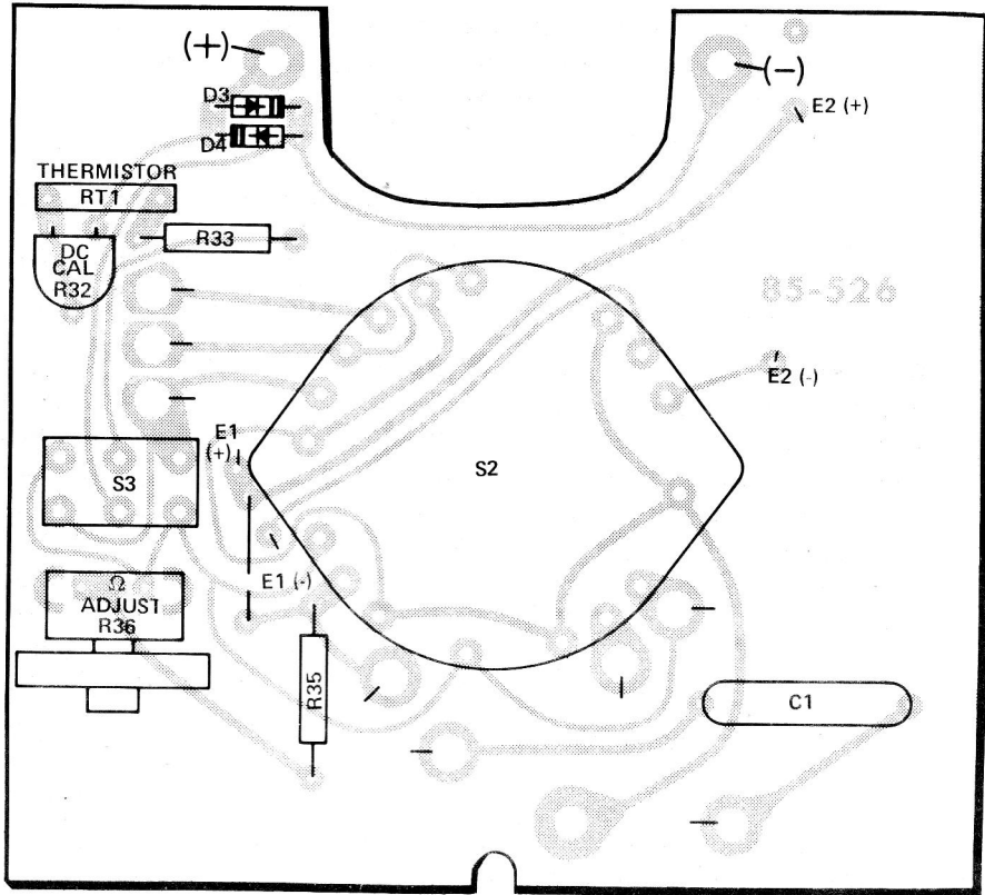
FRONT CIRCUIT BOARD (Shown from foil side)
