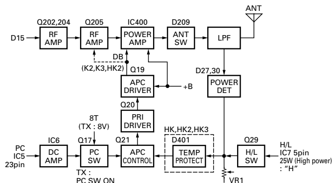
Fig. 8 APC circuit
