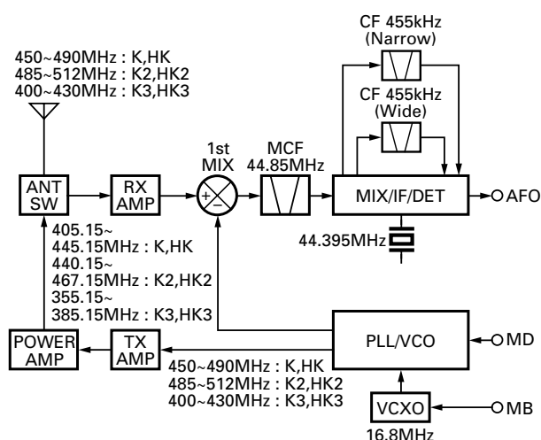
Fig. 1 Frequency configuration
